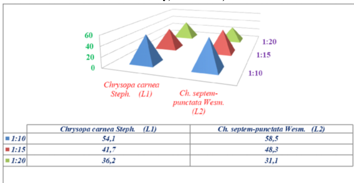
Figure 1. Effectiveness of aphidophages against aphids in poplar nursery (Sakson Ota State Forestry, 2019-2021)
